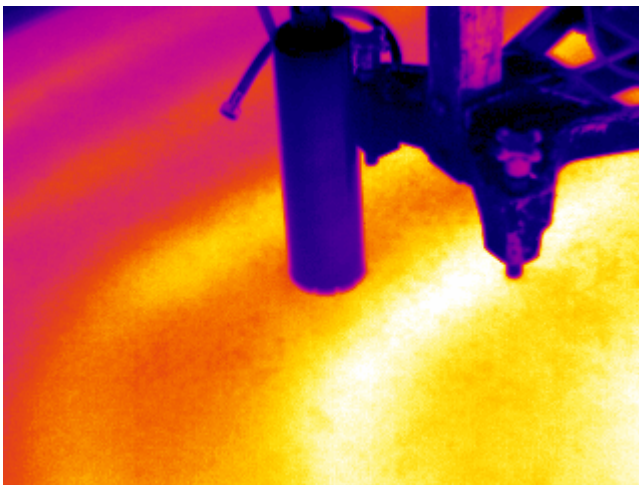
Figure 8. Concrete coring saw positioned between radiant heat lines to prevent damage to the system and subsequent leakage.
