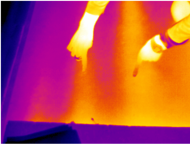
Figure 7. Radiant tubing locations identified in basement slab for purposes of slab coring and soil testing.
