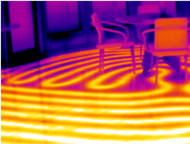
Figure 2. Dining area shown in Figure 1 begins to heat after several hours, however not to the rate of the adjacent floor section. Note that the infrared camera is also able to detect the radiant lines under marble flooring, as is the case with this image and Figure 1.
